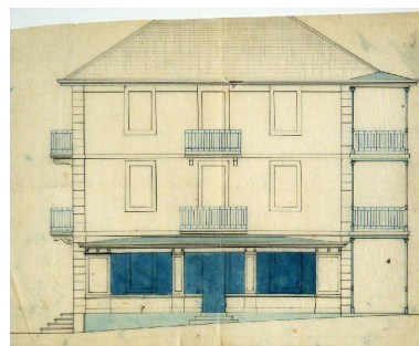
Elévation sud Repro. François Fouger IVR82_20047300242NUCB
