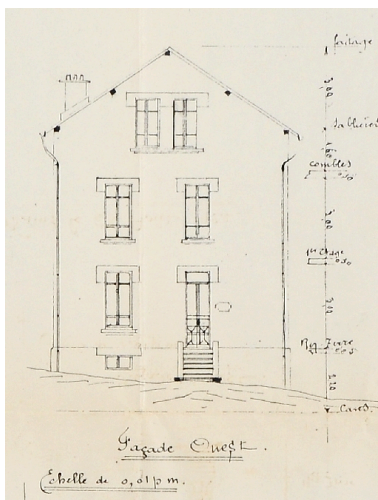
Elévation Repro. François Fouger IVR82_20097301060NUCB
