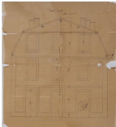
Élévation est, 1874 Repro. Denys Harreau IVR82_20157300273NUCB
