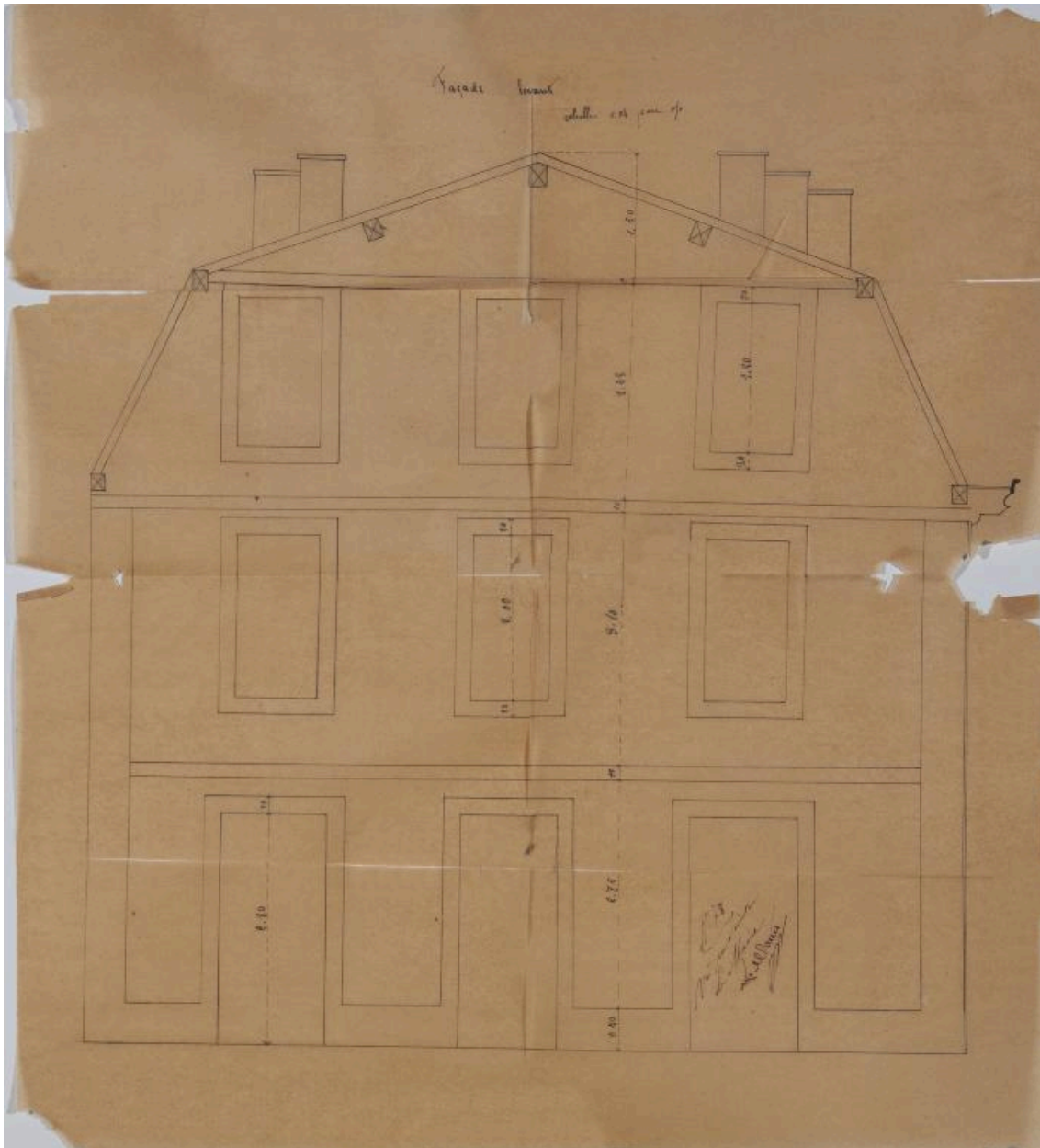
Elévation est, 1874
