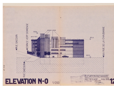
Elévations Repro. François Fouger IVR82_20057300748NUCB
