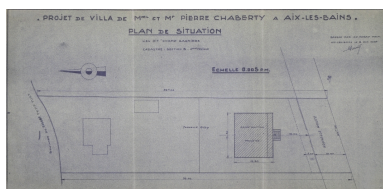
Plan de situation Repro. François Fouger IVR82_20127300381NUCB
