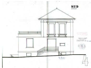
Elévation sud Repro. François Fouger IVR82_20077300859NUCB
