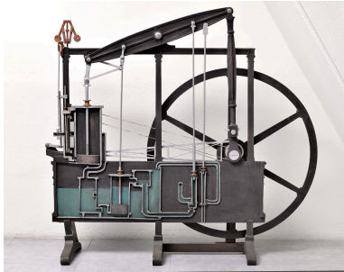
Machine de Watt, vue 1 Phot. Thierry Leroy IVR84_20256902017NUCA
