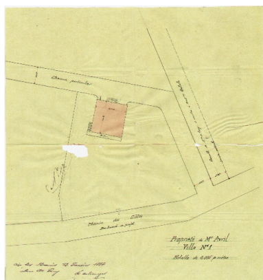
Plan masse, 1884 Repro. François Fouger IVR82_20127300693NUCB
