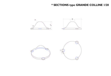
Section type Grande colline 1/20. Autr. Polly Brotherhood, Autr. Julia Maendler IVR84_20204200109NUDA
