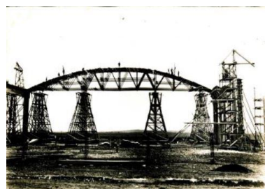
Hangar VI photo chantier ETs. Boussiron (ADR 1925 : 4535W47) Phot. Nadine Halitim-Dubois IVR84_20256900103NUC
