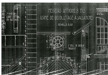
Plan usine Anthoine Phot. Nadine Halitim-Dubois IVR82_20057400013NUC
