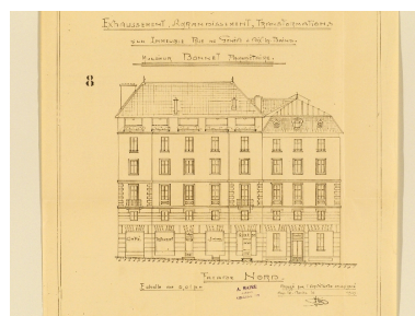
Elévation nord Repro. François Fouger IVR82_20087300152NUCB
