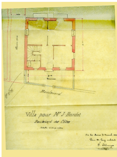
Plan Repro. François Fouger IVR82_20077300121NUCB
