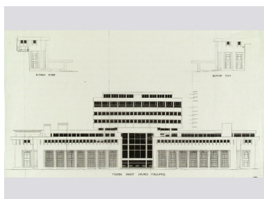
Elévation occidentale Repro. François Fouger IVR82_20067300182NUCB
