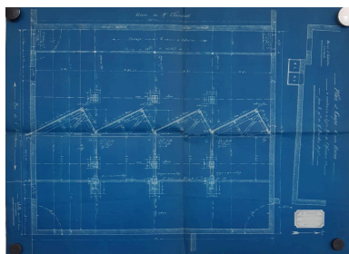
Plan extension usine 1907 (AC Lyon) Phot. Nadine Halitim-Dubois IVR84_20196900141NUCA
