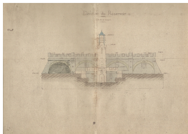
Elévation Repro. François Fouger IVR82_20087300790NUCB
