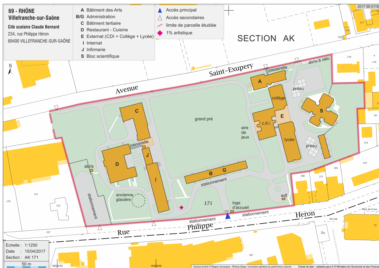
Plan-masse
