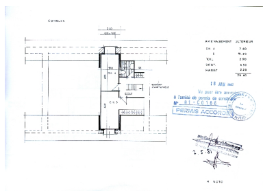
Plan des combles Repro. François Fouger IVR82_20097300326NUCB
