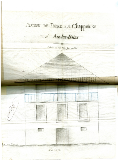
Elévation principale Repro. François Fouger IVR82_20097300329NUCB
