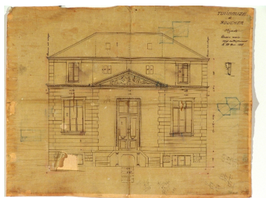
Elévation principale Repro. François Fouger IVR82_20057300063NUCB
