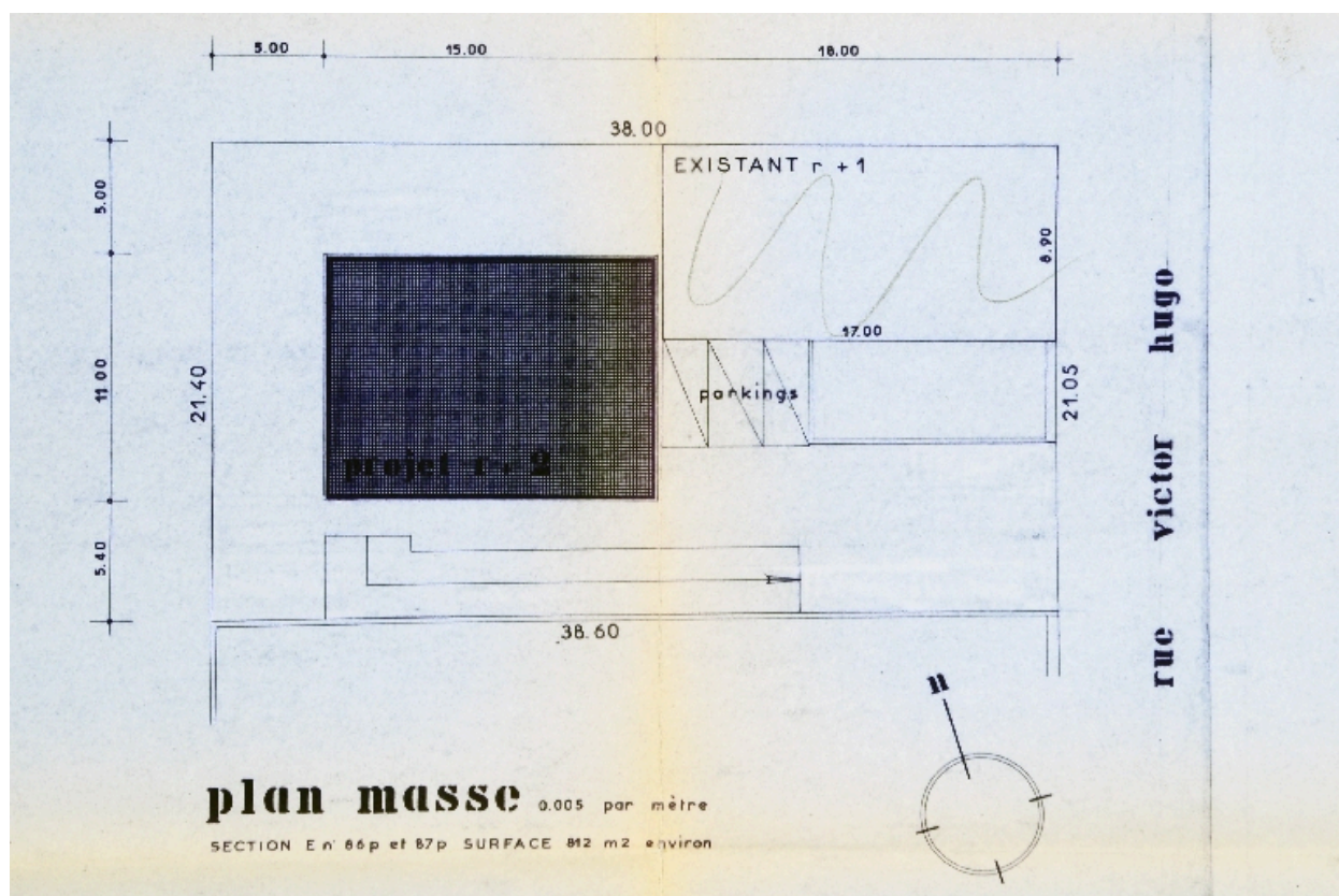
Plan-masse
