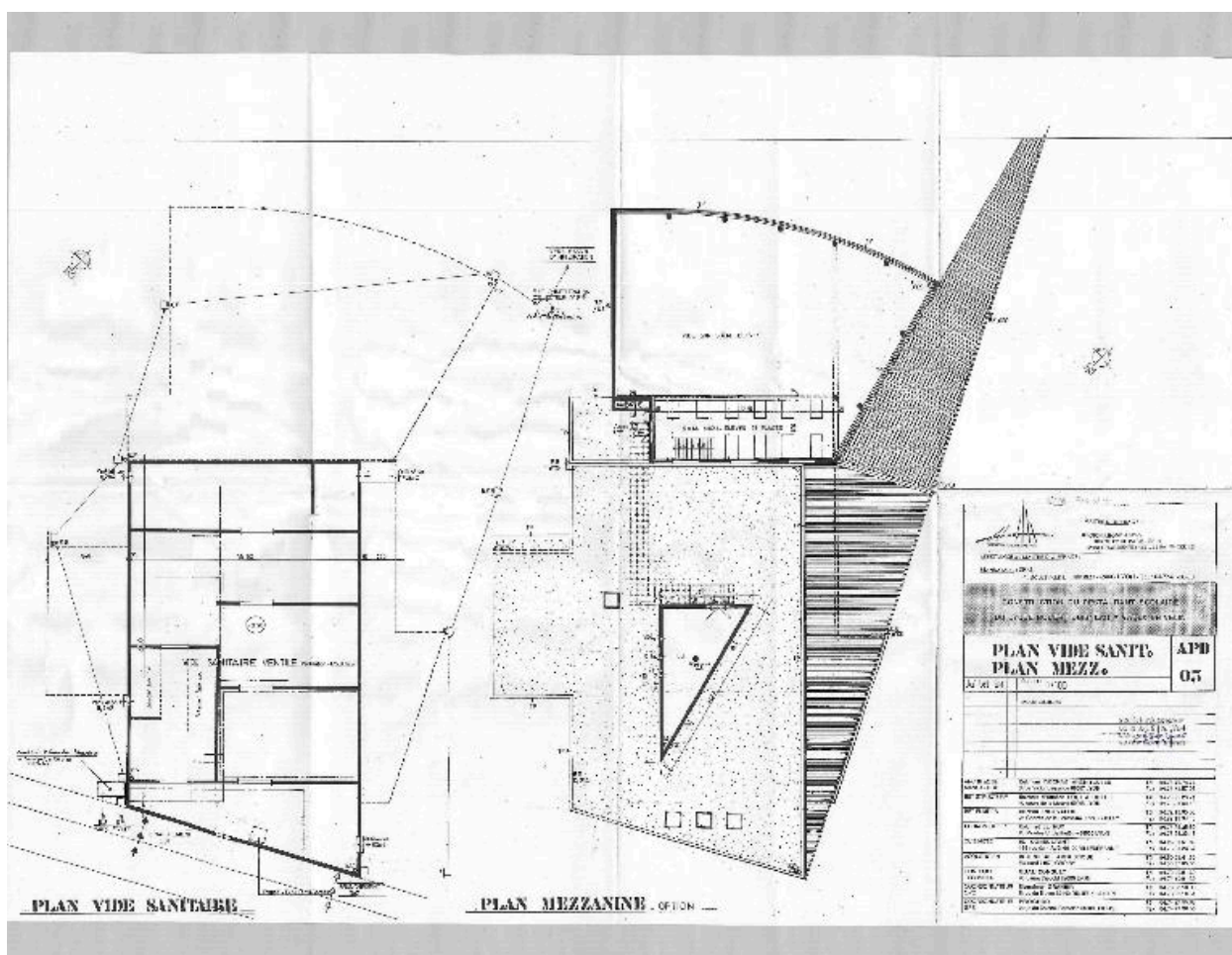
Construction du restaurant scolaire. Plan vide sanit. Plan Mezz. (1998)
