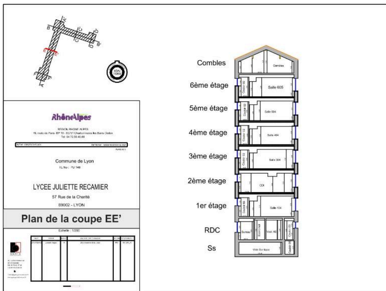
Coupe EE'. Dess. AGATE, 2012
