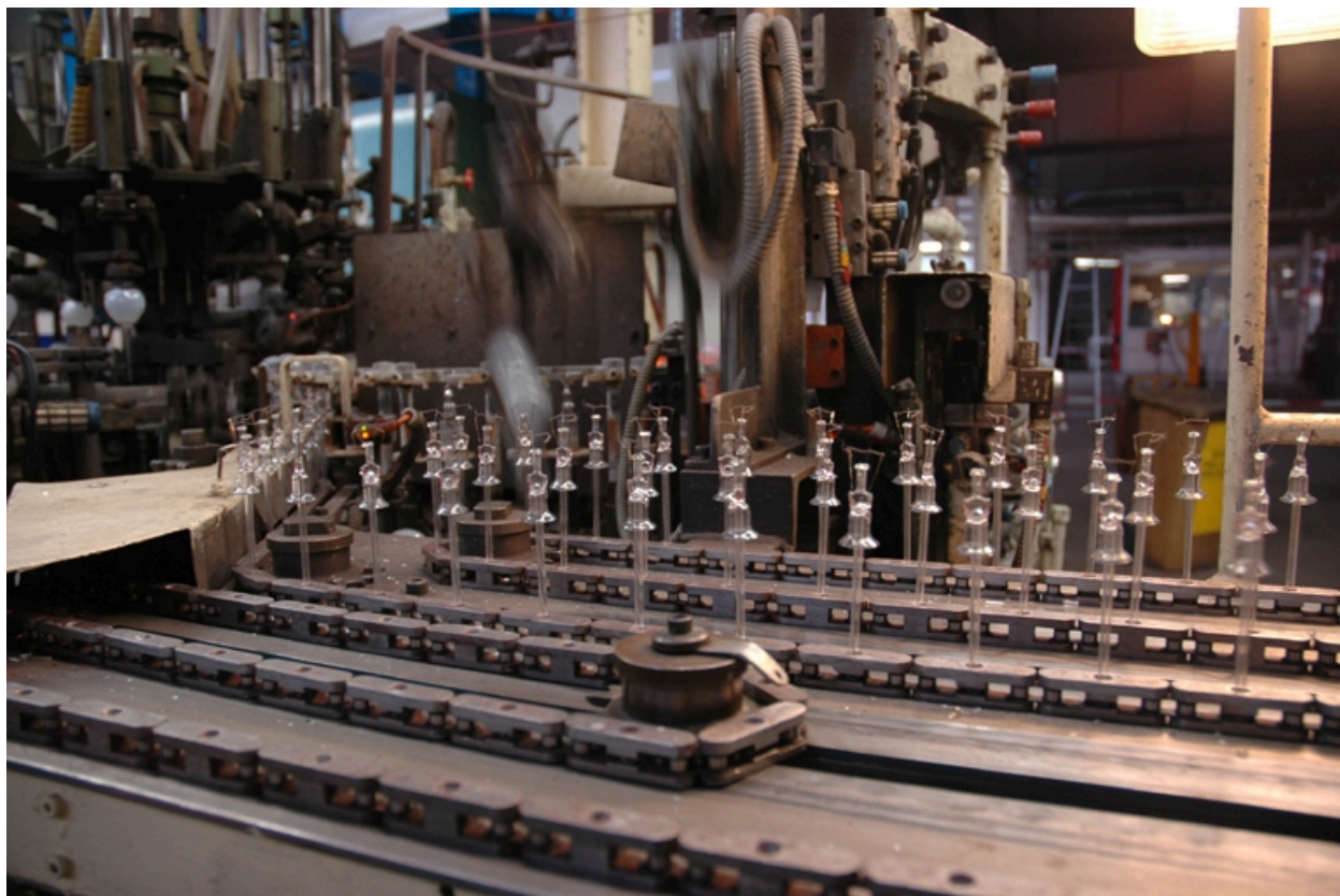
Machine pied-filament
