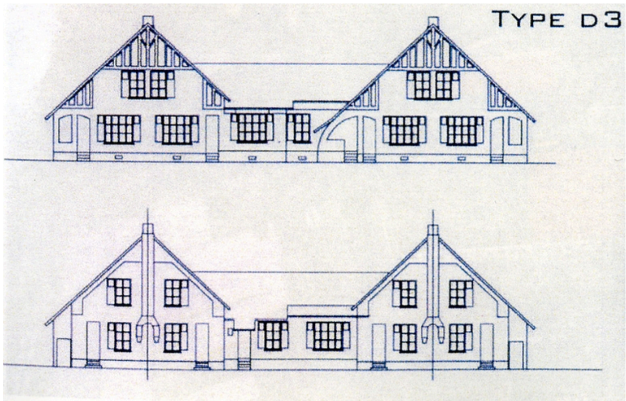
Plan façade
