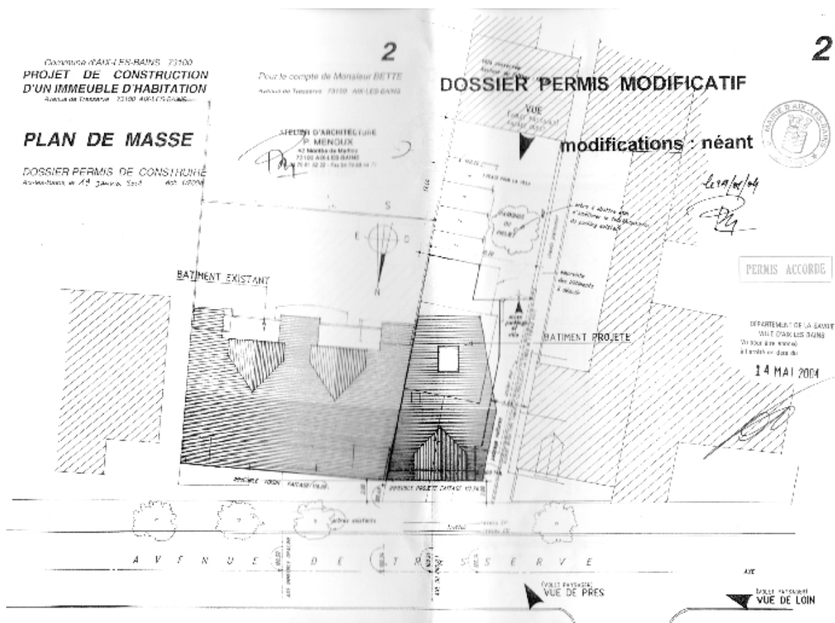
Plan-masse
