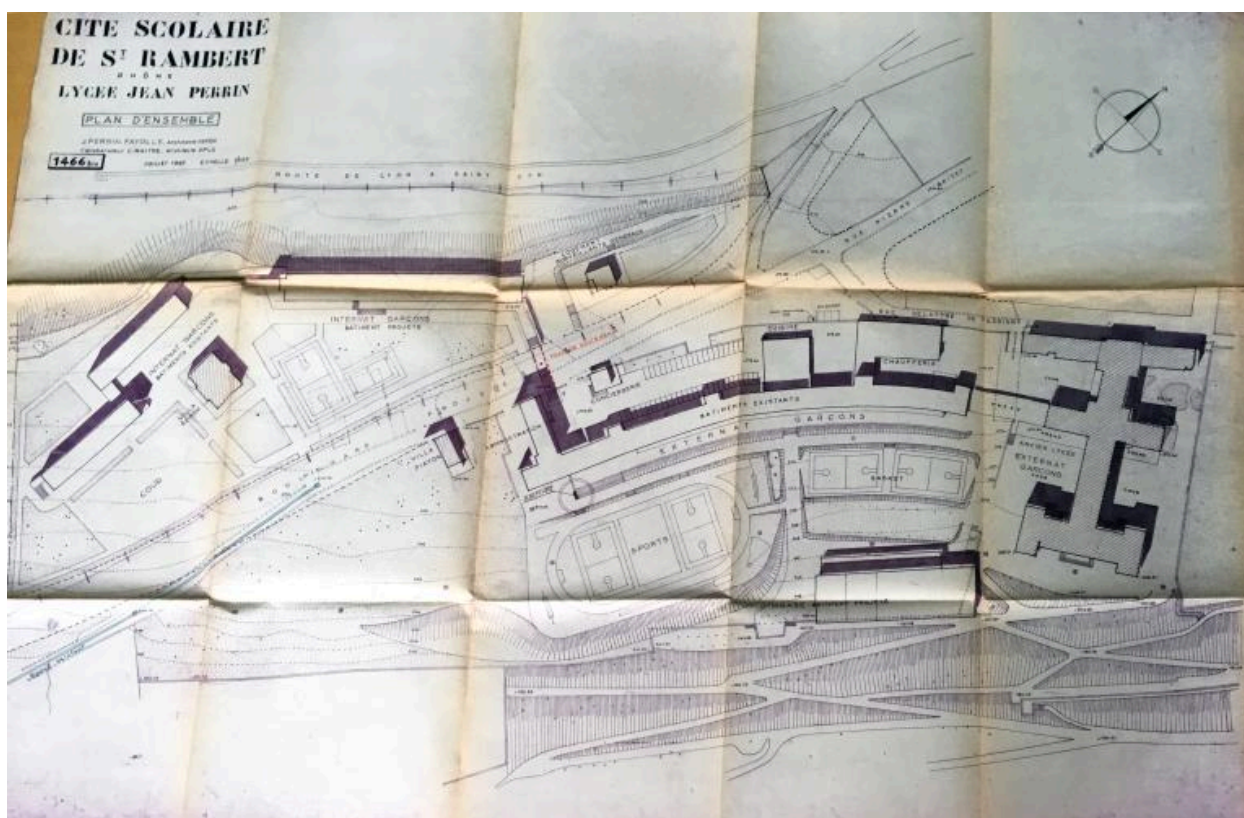
Plan masse, 1961 (AC Lyon, 472 WP 57)
