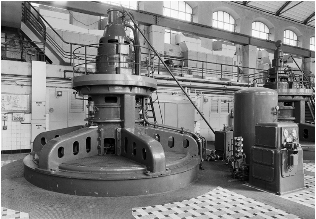
Turbine G8, Alsthom usine de Belfort
